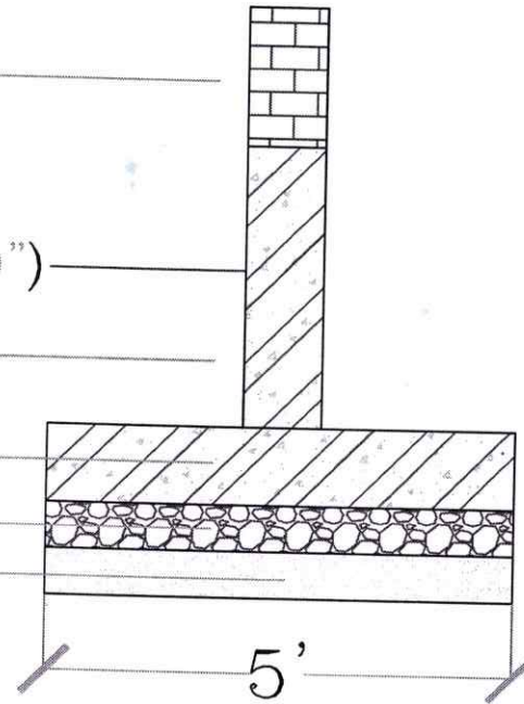
Sectional View
