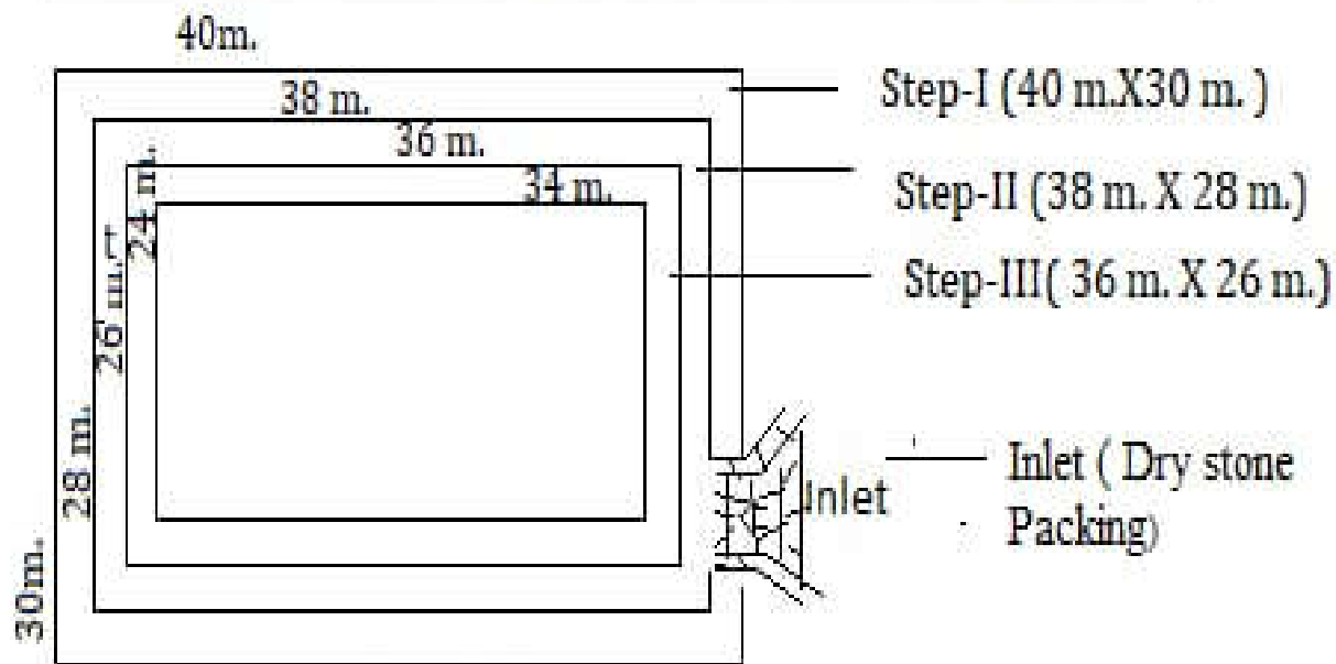
(Plan of Water Body)
